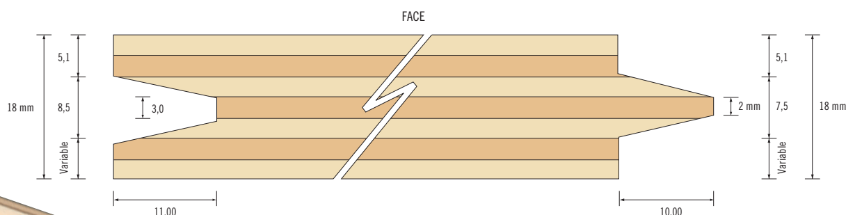
18 mm T&G-M EDGE PROFILE DIAGRAM
